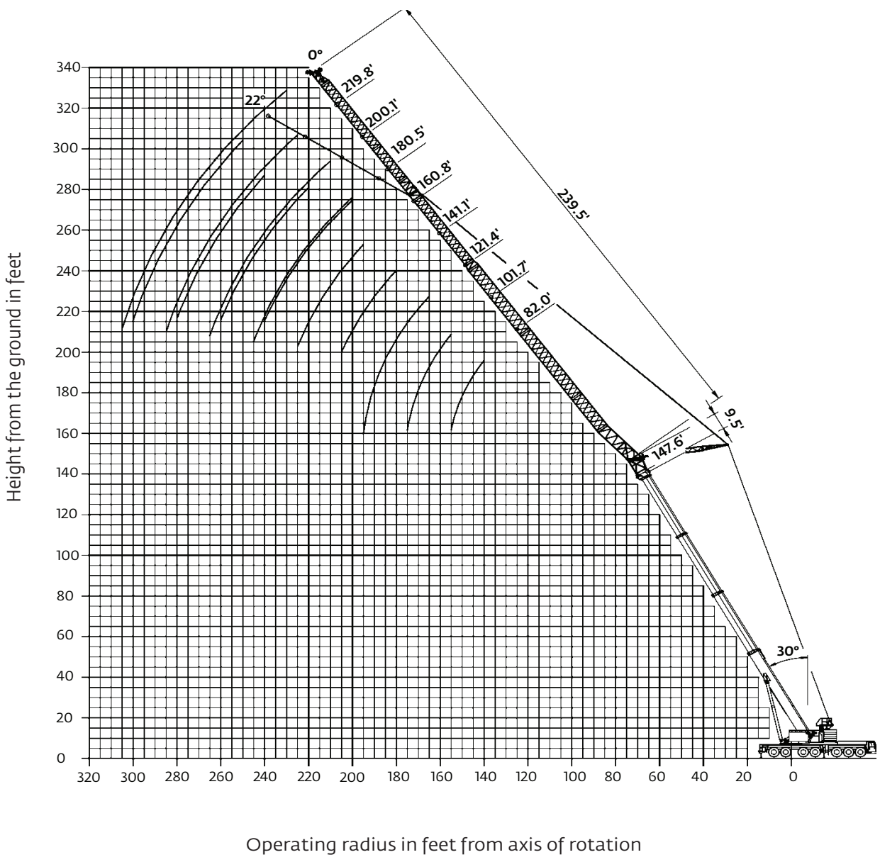
82 ft - 240 ft luffing jib - 60° main boom
