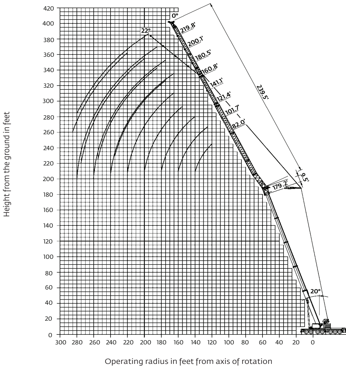
82 ft - 240 ft luffing jib - 70° main boom
