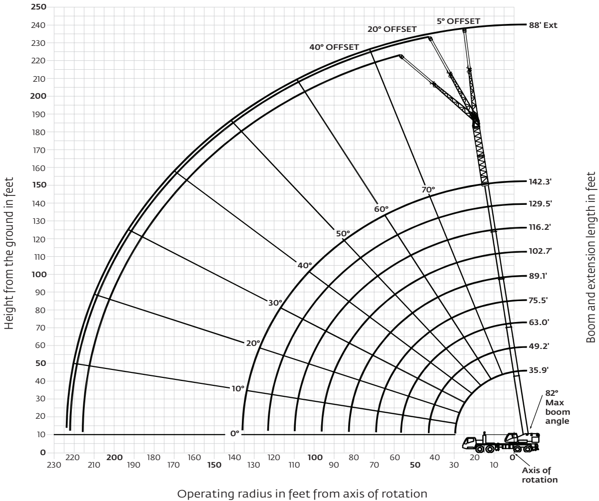
33 ft -56 ft hydraulic lattice extension with two 16 ft inserts
