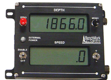
BACKUP PANEL DEPTH / SPEED BUILT-IN DATA RECORDER
