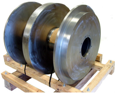
FSU1M856 SPLIT DRUM 38" X 13.9" EQUAL SPLIT X 12.4" CORE 26.4K' 7/32" X 2 12.7K' 5/16" X 2
