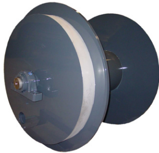
DEEP WELL CASED HOLE DRUM 40,000 FEET - 7/16"
